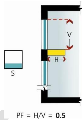
Figure 4.33 PF for south interior light shelf
