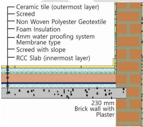
RCC slab with insulation
