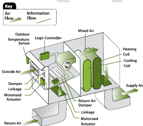
Figure 5.16 Economizer
